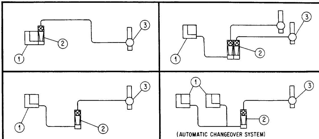
1. VACUUM REGULATOR 2. FLOWMETER AND RATE VALVE 3. EJECTOR SI-5462
